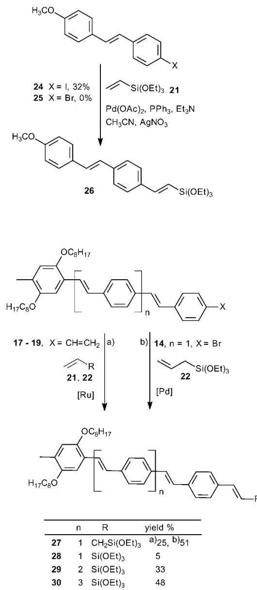
Scheme 3. Synthesis of alkoxysilyl-substituted OPVs; a) cross-metathesis: [Cl 2 (PCy 3 ) 2 Ru=CHPh], benzene, ambient temperature; b) Pd(OAc) 2 , P( o -tol) 3 , Et 3 N, DMF, 100 °C.
