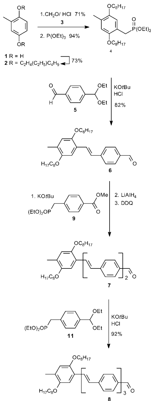
Scheme 1. Synthesis of OPV-aldehydes 6–8 .
