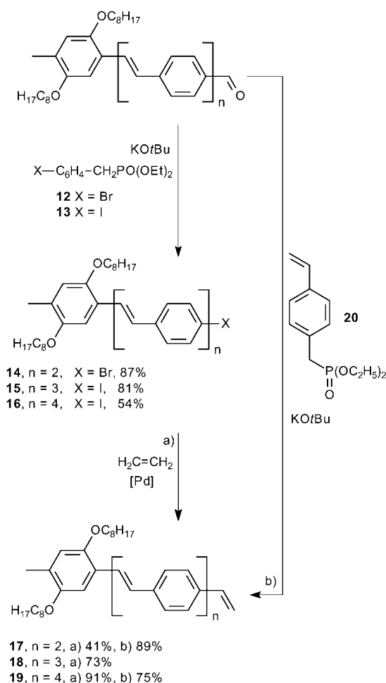
Scheme 2. Heck and Horner reactions to vinyl-substituted OPVs 17–19 .
